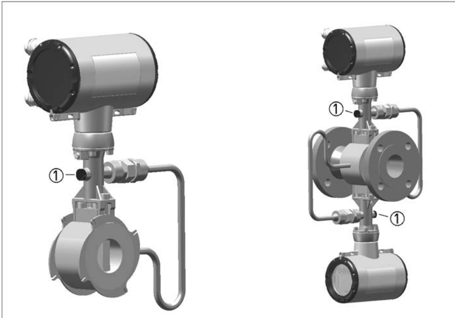
Figure 2-7: Dual Seal
