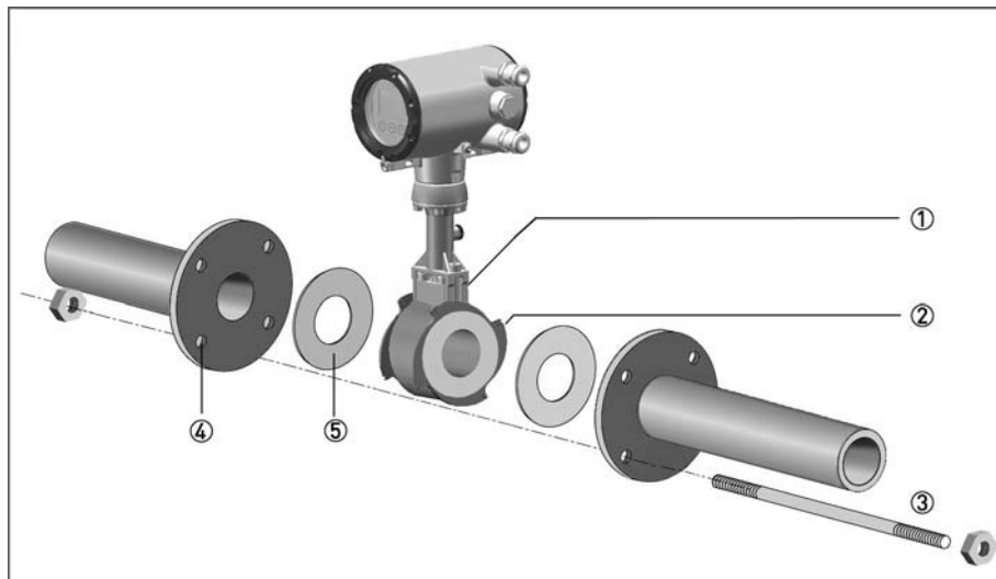
Figure 3-12: Installation using centering ring
