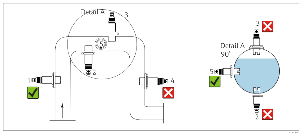
9 Permitted and unacceptable orientations in pipes
