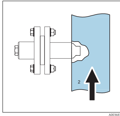
12 Installing with CUA120 flow assembly
