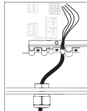
8 Tightening the screw (2 Nm (1.5 lbf ft))
