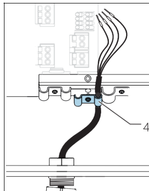
7 Inserting the cable
