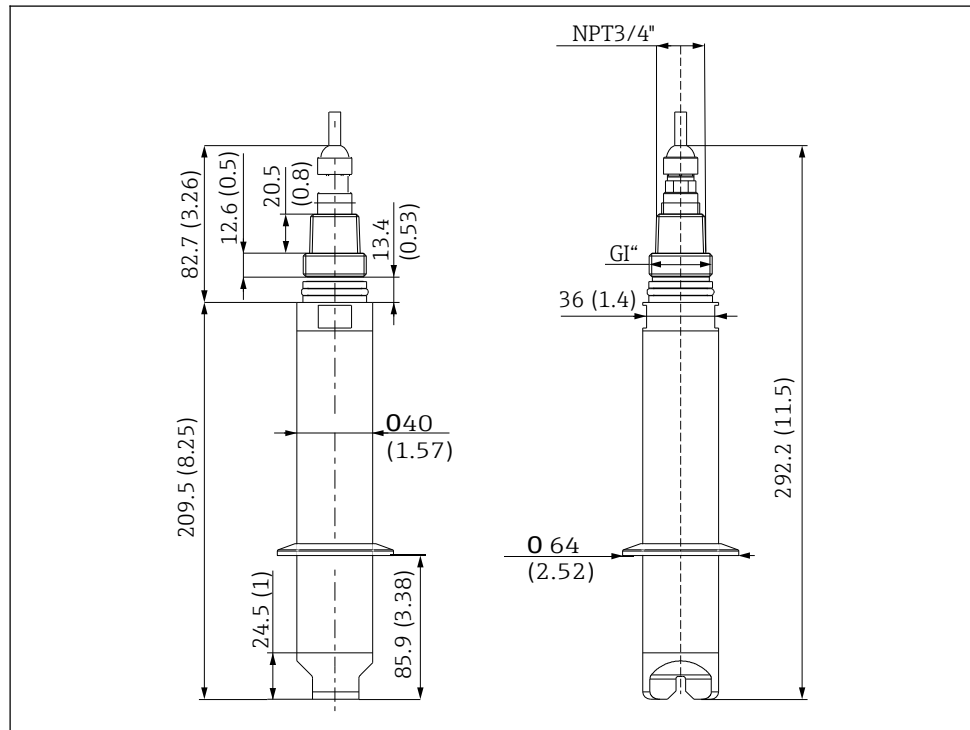
19 Dimensions with clamp. Dimensions: mm (in)
