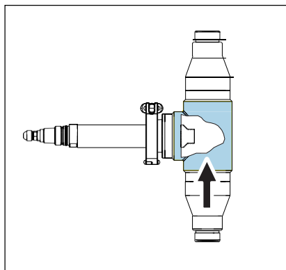
13 Installing with CUA252 flow assembly
