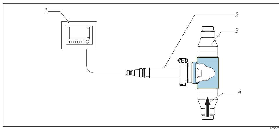
1 Measuring system with CUA252 flow assembly
