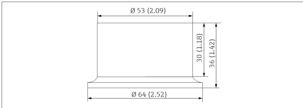
21 Weld-in adapter. Dimensions: mm (in)
