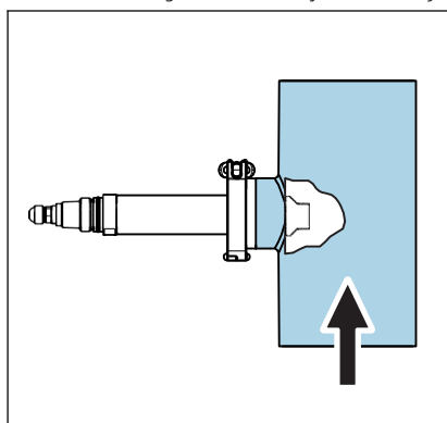
14 Installing with CUA262 flow assembly
