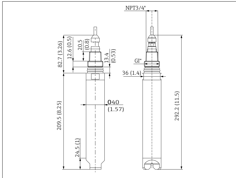
18 Dimensions. Dimensions: mm (in)
