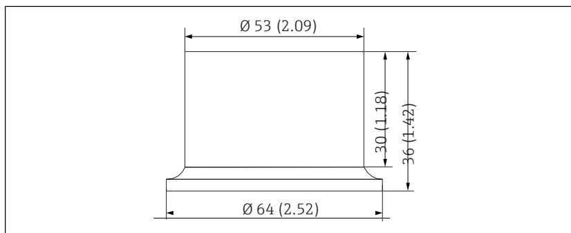
21 Weld-in adapter. Dimensions: mm (in)
