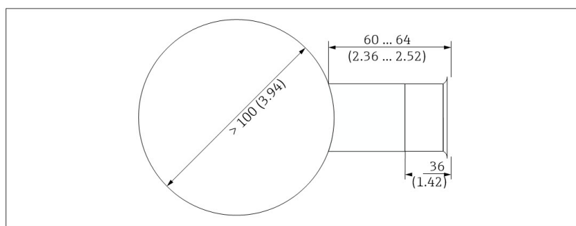
22 Pipe connection with weld-in adapter. Dimensions: mm (in)
